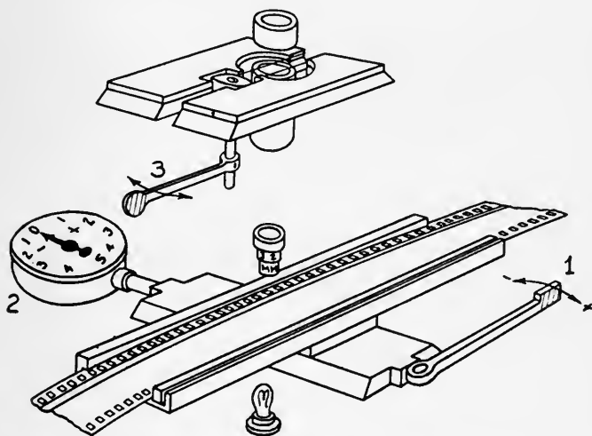
FIG. 1. Schematic arrangement of device.
